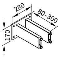
stand-off bracket 80-300 mm incl. insulating element
